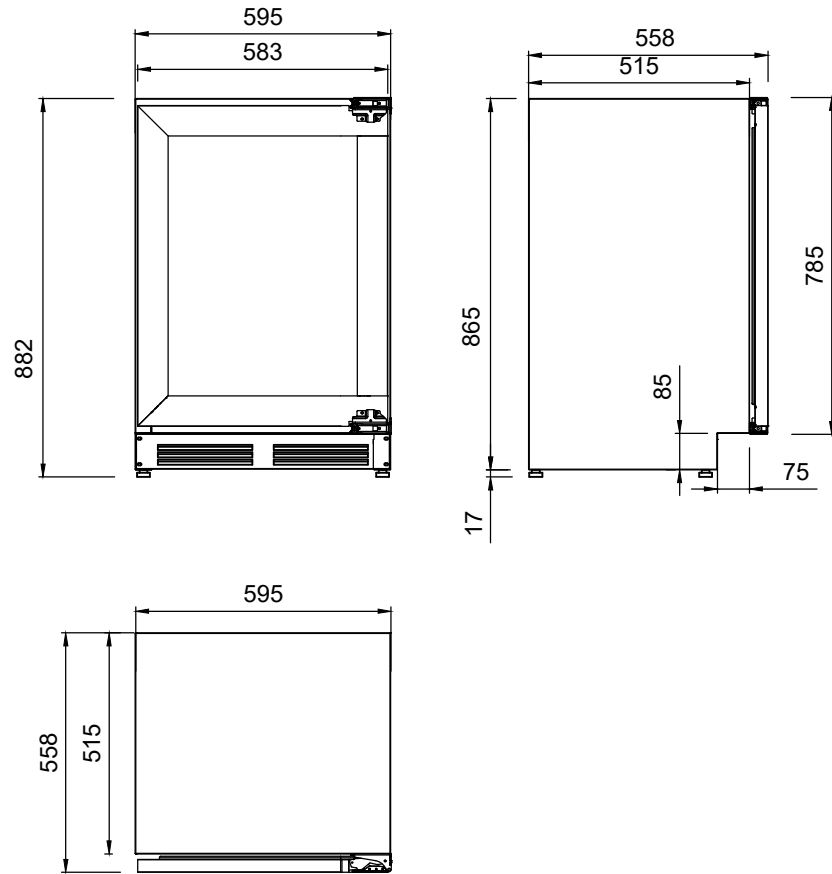
WU6088H-2P46 with normal legs
