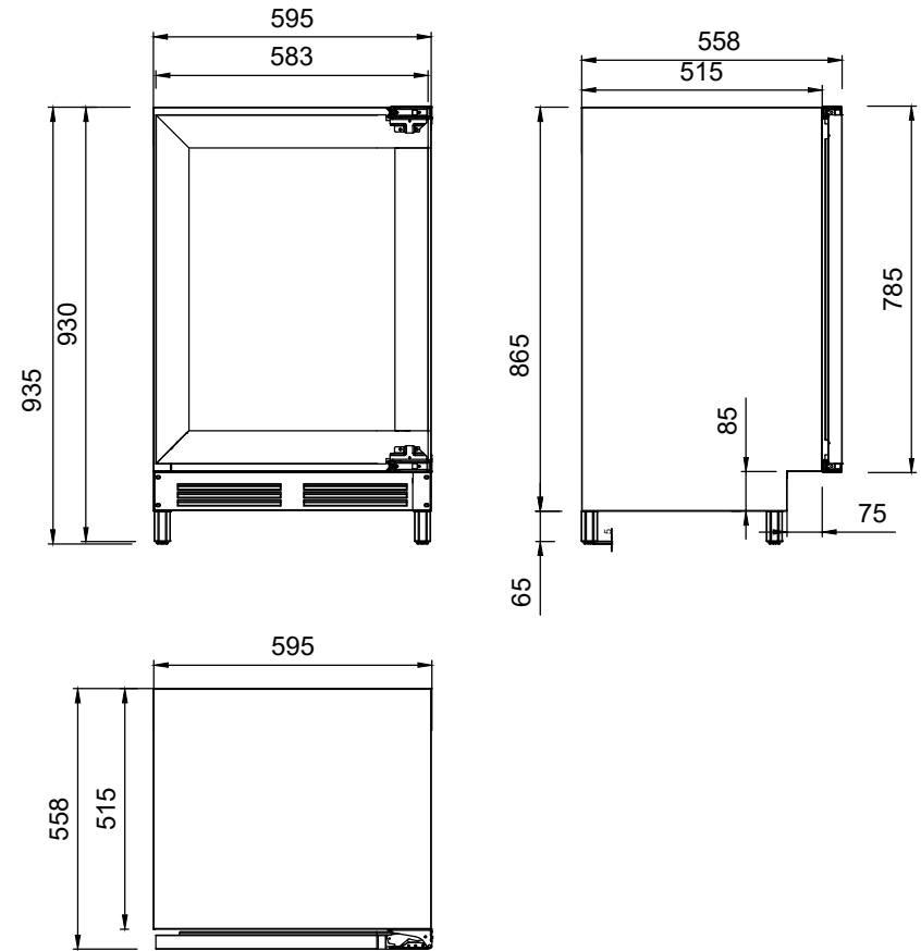
WU6088H-2P46 with taller legs
