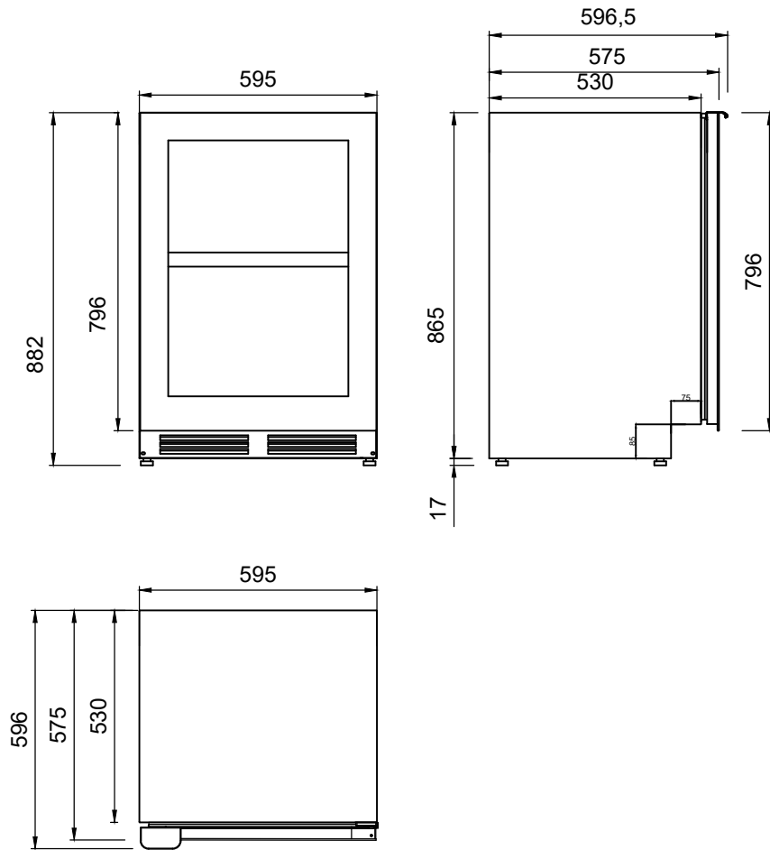
WU6088H-2B46 WU6088T-2B46 with normal legs door: 796mm high
