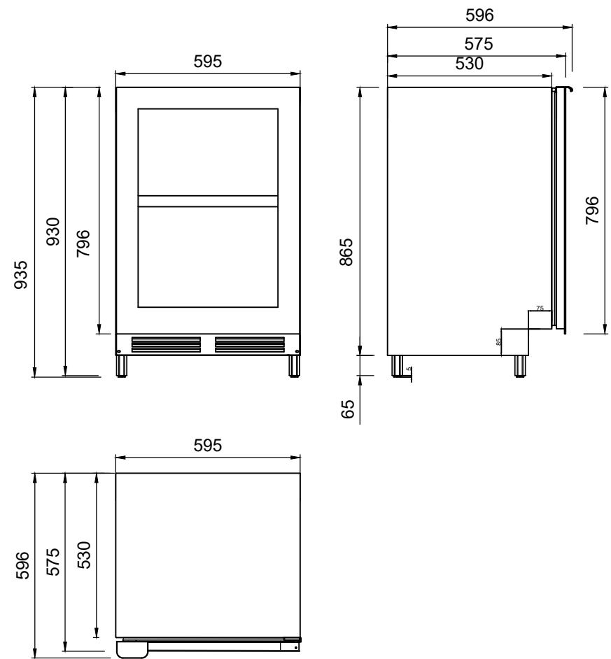
WU6088H-2B46 WU6088T-2B46 with taller legs door: 796mm high
