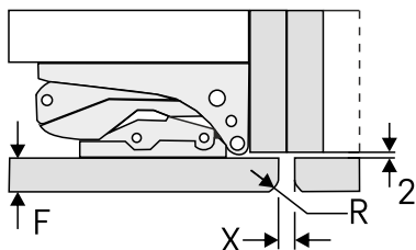
Fig. 68 Joint gap with adjoining unit door
