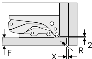
Fig. 67 Joint gap with adjoining furniture side panel
