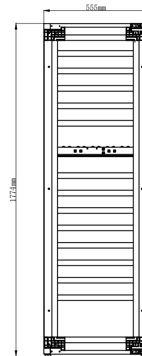
Front View
